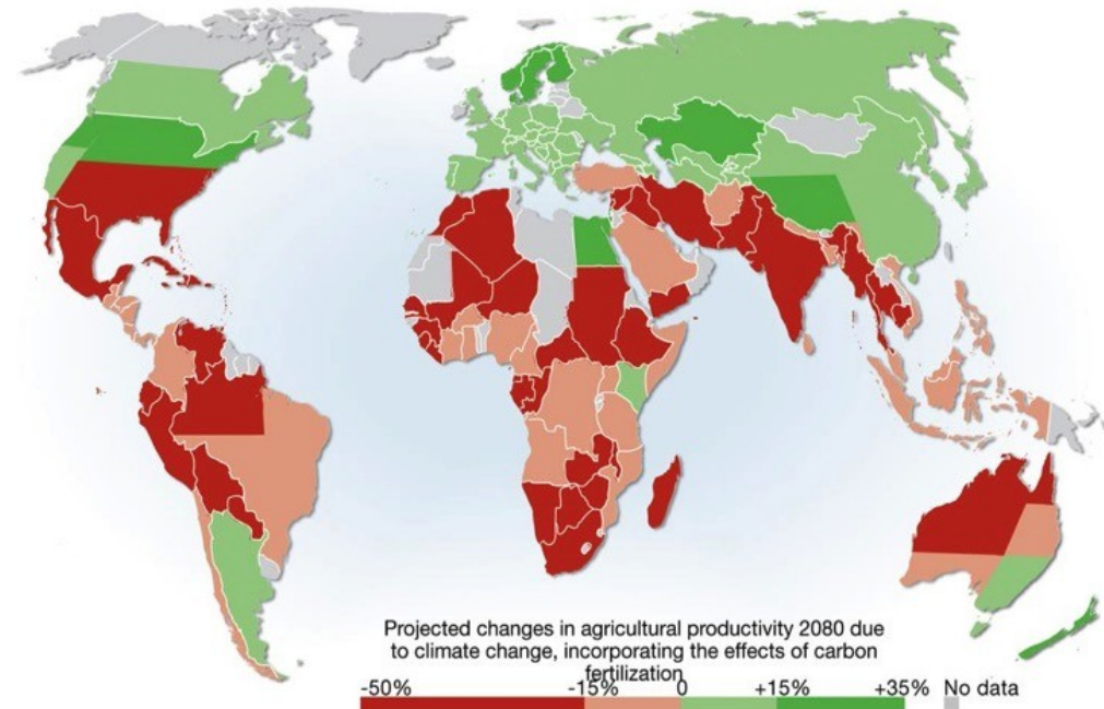
Projected changes in agricultural productivity 2080 due to climate change, incorporating the effects of carbon fertilization (Ahlenius, 2009)
